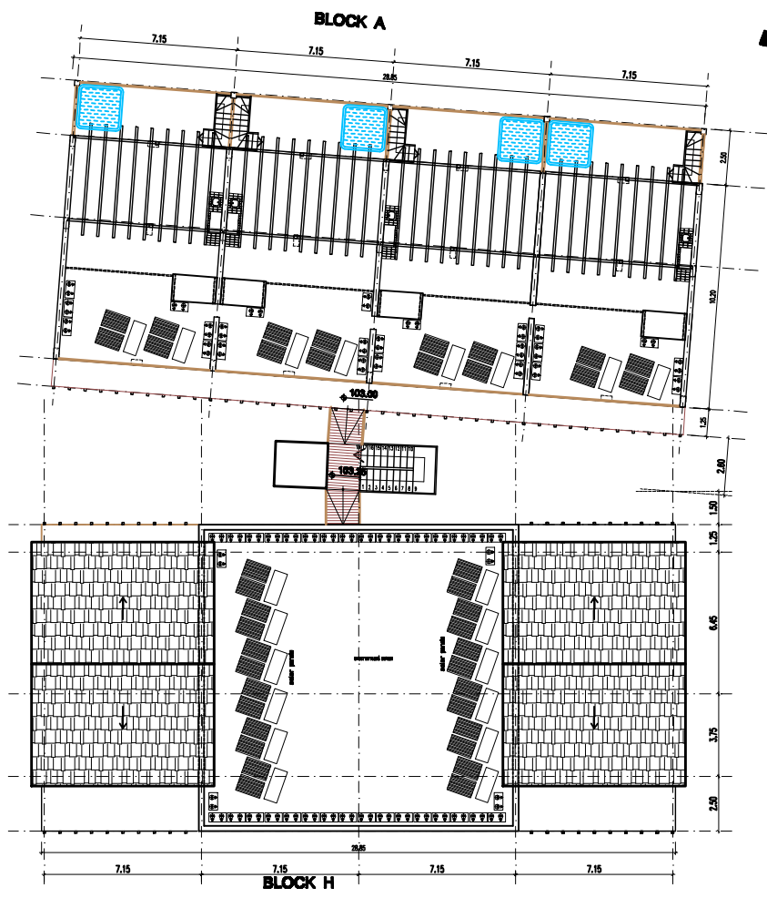
ROOF PLAN
